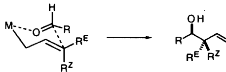
Scheme 2. Chair-like six-membered cyclic transition state
